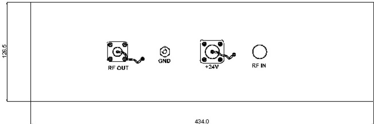
REAR VIEW
