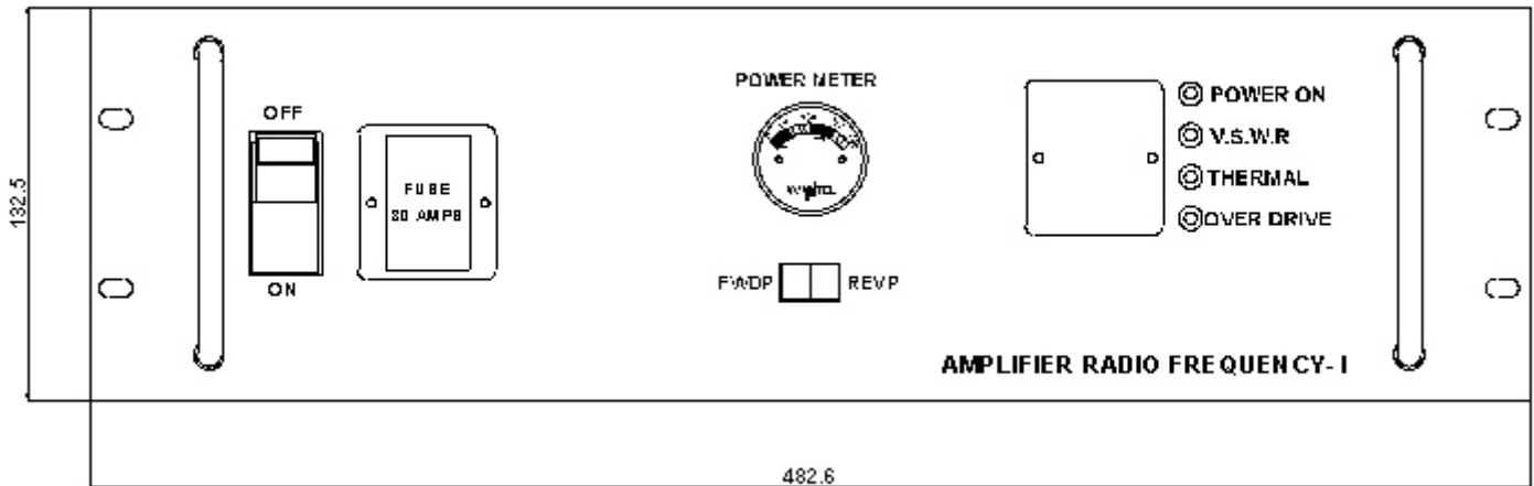
FRONT VIEW
